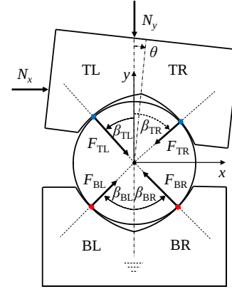
Figure 6. Contact force model
