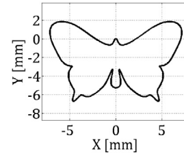
Fig. 5. Desired path.
