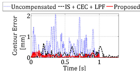
Fig. 9. Contour errors for uncompensated, IS + CEC + LPF and proposed (optimal) trajectories.
