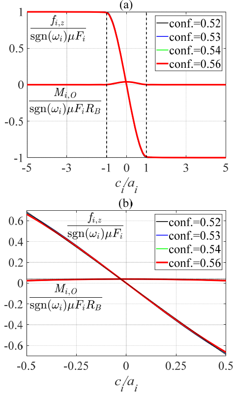
Figure 4. Frictional force and moment as functions of c/a_i : (a) full plot; (b) zoomed in plot near c/a_i = 0
