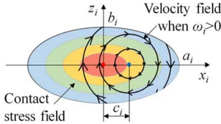
Fig. 3 Contact area and relative velocity field for linear ball bearing
