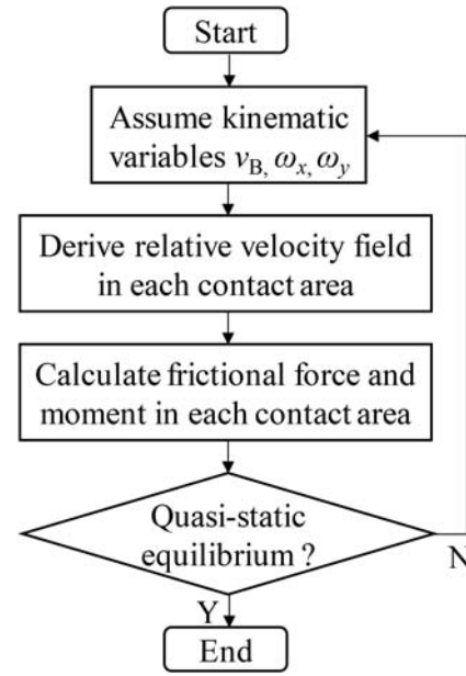
Fig. 4 Flowchart for the solving process of ball motion and friction in linear ball bearing
