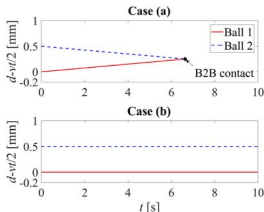
Fig. 10 Example of ball-to-ball contact and its avoidance by optimized design
