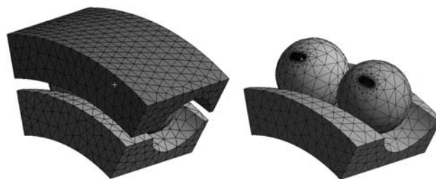
Fig. 18 Mesh for ball screw in ANSYS
