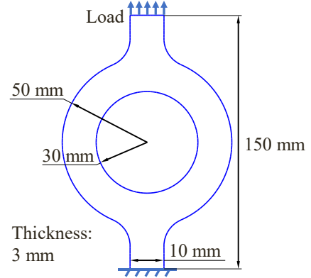
Fig. 10. The loop-shaped specimen and loading conditions.
