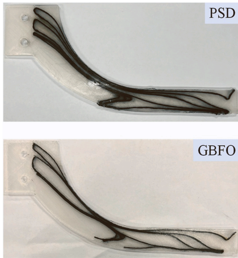
Fig. 23. The beams with fiber paths generated from the PSD and the GBFO methods.
