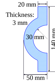
Figure 5: The Geometry of Half Loop
