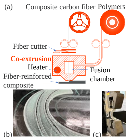
Figure 9: (a) Working Principle of the 3D Printer, (b) Fiber Path Detail, and (c) The MTS Sintech 10/D Fixture with the Half Loop
