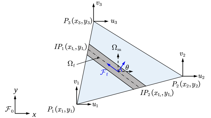
Figure 1: Three-Node Triangular Element with Fiber
