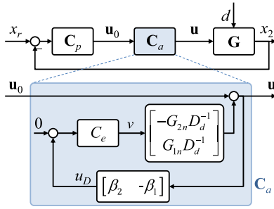
Fig. 2. Block diagram of the two-stage control framework using PBCA.
