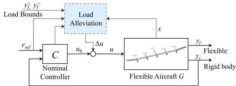
Fig. 1 Block diagram of maneuver load alleviation with the nominal controller
