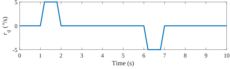
Fig. 4 Pitch rate reference trajectory of GTA
