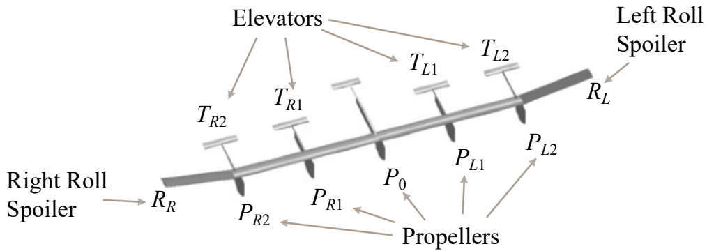
Fig. 8 Schematics of X-HALE
