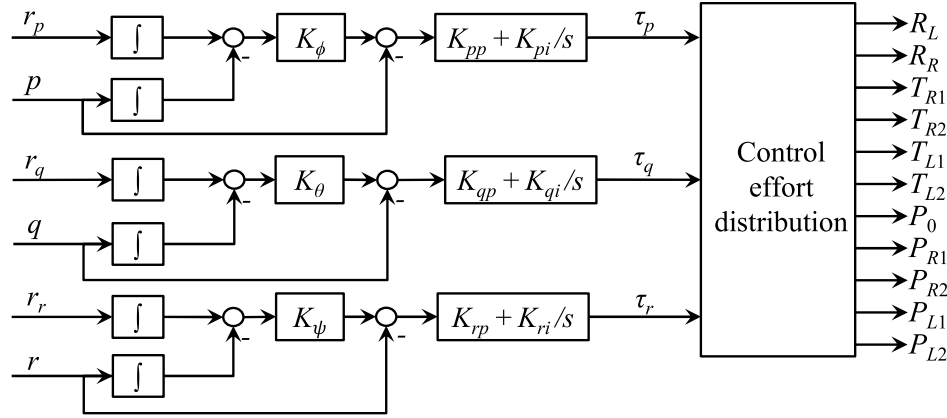
Fig. 10 Nominal controller C structure
