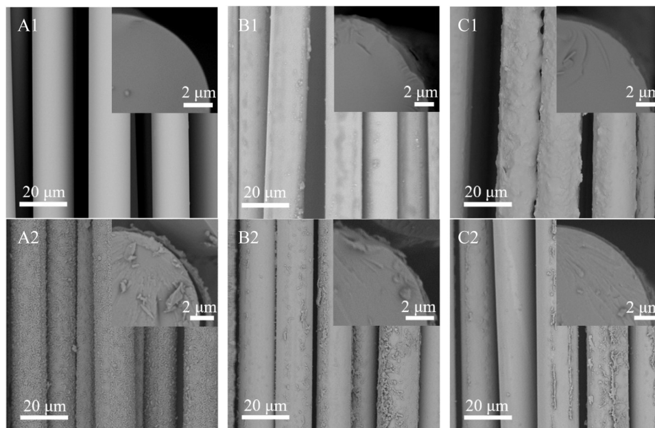
Fig. 9. Morphology of BF before and after seawater treatment (A: Without sizing; B: With epoxy sizing; C: With nanocomposite sizing; 1: Untreated; 2: Seawater-treated; Insets showing the cross-sectional morphology of corresponding sample).
