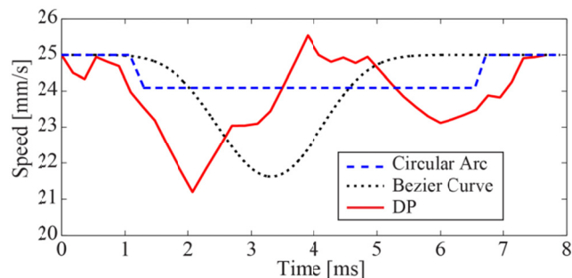
Figure 7. COMPARISON OF SPEED PROFILES FOR OBTUSE-ANGLED CORNER
