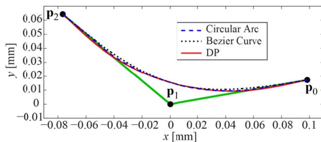
Figure 7. COMPARISON OF CORNER PATHS FOR OBTUSE-ANGLED CORNER
