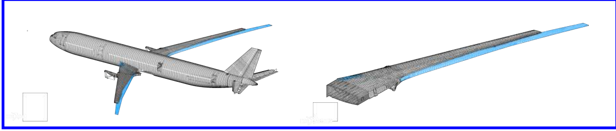
Fig. 4 Comparison of the XRF1 (black) and XRF1-HARW (blue) wing box and body [22]
