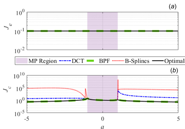
Fig. 3 Effect of basis functions (DCT, BPF, B-splines, and Optimal) on (a) J_e and (b) J_c for various values of a ( M = 1000 , n = 990 )
