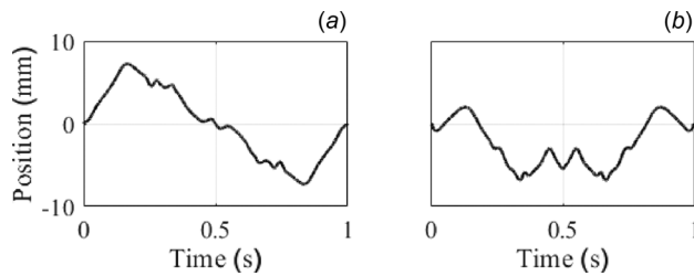
Fig. 10 Desired position trajectories along the X- and Y-axes: (a) x-axis and (b) y-axis
