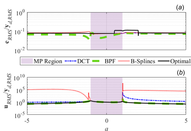
Fig. 4 Effect of basis functions (DCT, BPF, B-splines, and optimal) on (a) normalized RMS tracking error, e_{\text{RMS}}/y_{d,\text{RMS}} and (b) normalized RMS control input for various values of a ( M = 1000 , n = 990 ), u_{\text{RMS}}/y_{d,\text{RMS}}
