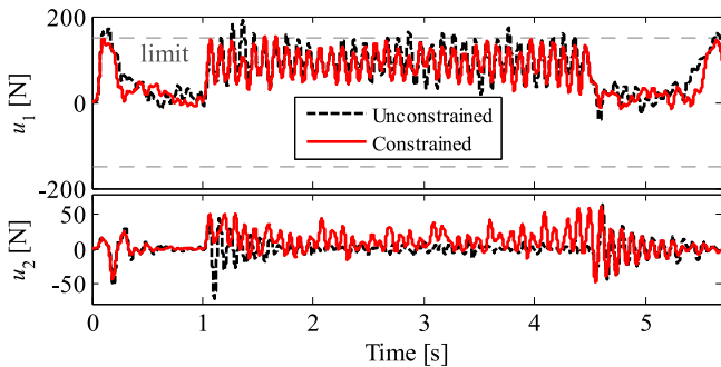
Fig. 10. Comparison of control efforts of proposed proxy-based dynamic allocator with and without constraints, low-pass filtered with 16 Hz cutoff.
