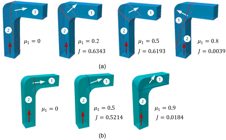
Fig. 9. Optimized SESEVD solution for L-shaped beam with specific \mu_1 under (a) single-loading and (b) multiple-loading conditions.
