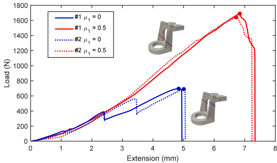
Fig. 15. Comparison of bending test results between the SESEVD optimized and non-optimized group on the mechanical mounter.
