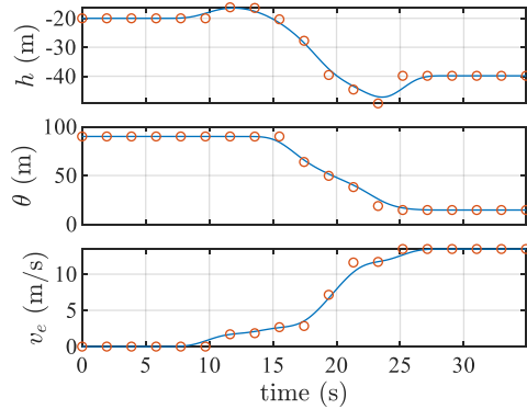
Fig. 7 Optimized ETS-20 transition trajectories of height h , pitch \theta , and ground speed v_e
