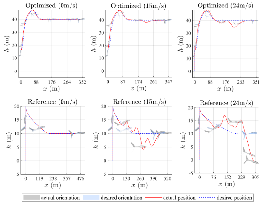
Fig. 8 Aircraft position compare under 0m/s, 15m/s, and 24m/s gust
