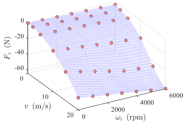
Fig. 4 Propeller-wing slipstream database
