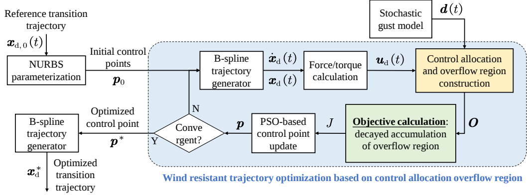
Fig. 2 Wind resistant transition trajectory optimization procedure
