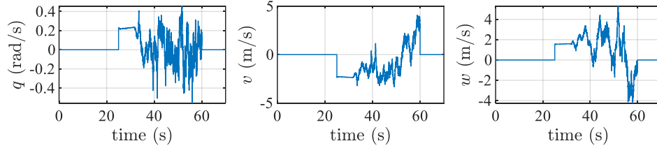
Fig. 5 Von Karman gust (24 m/s)'s effectiveness on pitch velocity q , x-axis velocity v , and z-axis velocity w
