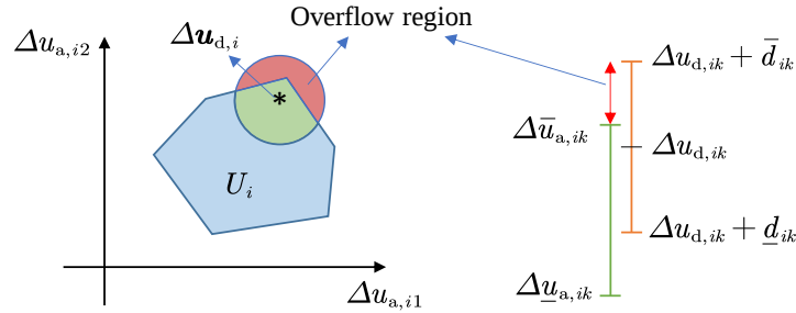
Fig. 1 Margin and attainable subset of input increment
