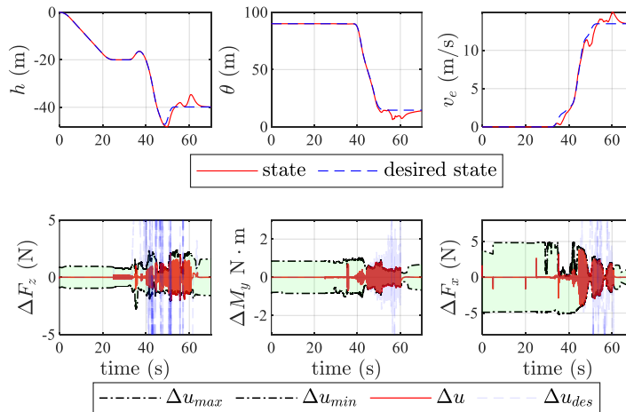
Fig. 9 Aircraft height, pitch, ground speed, and attainable subset under 24 m/s Von Karman gust
