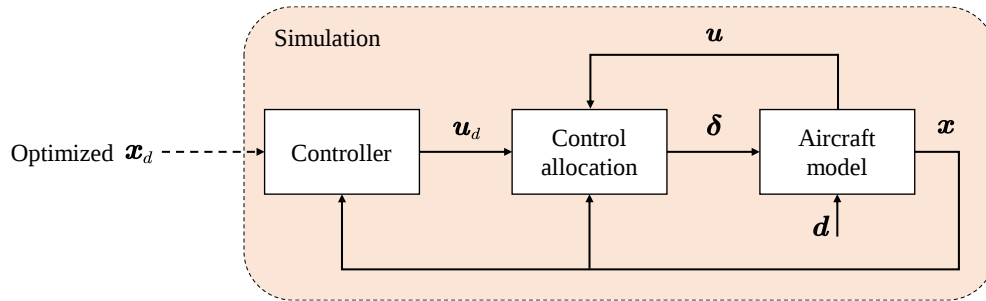
Fig. 6 Aircraft control block diagram based on backstepping control and control allocation
