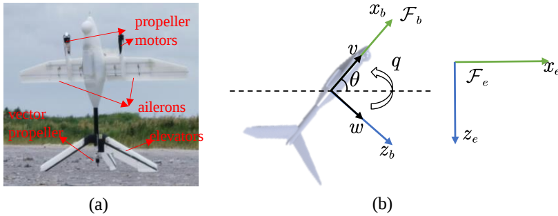
Fig. 3 Prototype ETS20 for case study (a) and the notations of states (b)
